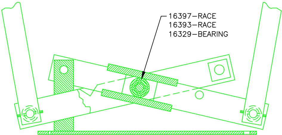
HEAD CLOSING SYNCHRONIZER SECTION
